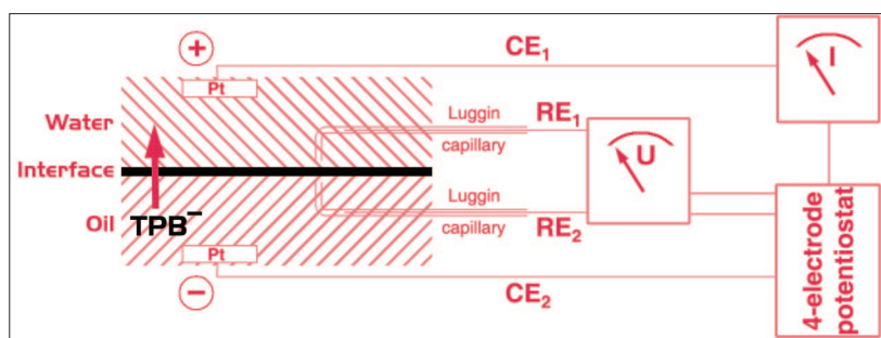
Diagram of the electrochemical cell used in the liquid–liquid interface experiments. A brochure describing his research is available directly from the author and on his personal Web page, www.vanysek.com/electrochem/ .
